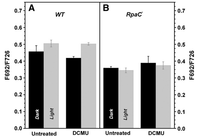
Fig. 2. The ratio of the 77 K fluorescence maxima, F692/F726 (Photosystem II/Photosystem I), measured with WT (A) and RpaC - mutant (B) of Synechocystis sp. PCC 6803. Fluorescence excitation, \lambda_e = 530 nm, \Delta\lambda = \pm 20 nm (green diode), standard deviation bars are for n = 3 . Ratios were obtained after curve deconvolution; other details are as in Fig. 1 legend.
