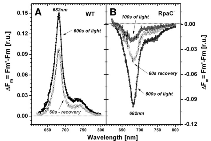
Fig. 7. Fluorescence difference spectra (illuminated minus dark) of maximal fluorescence for WT (A) and RpaC - mutant (B) of Synechocystis sp. PCC 6803. Data were calculated from numbers obtained from SRFI plots for wild-type cells (Fig. 4) and RpaC - mutant cells. \Delta F_m is the difference between F_m' and F_m , where F_m is the maximal fluorescence measured in dark and F_m' is the maximal fluorescence measured after a particular time of irradiation and after 60 s of recovery in dark (60 s recovery). Data represent average curves from n = 4 .
