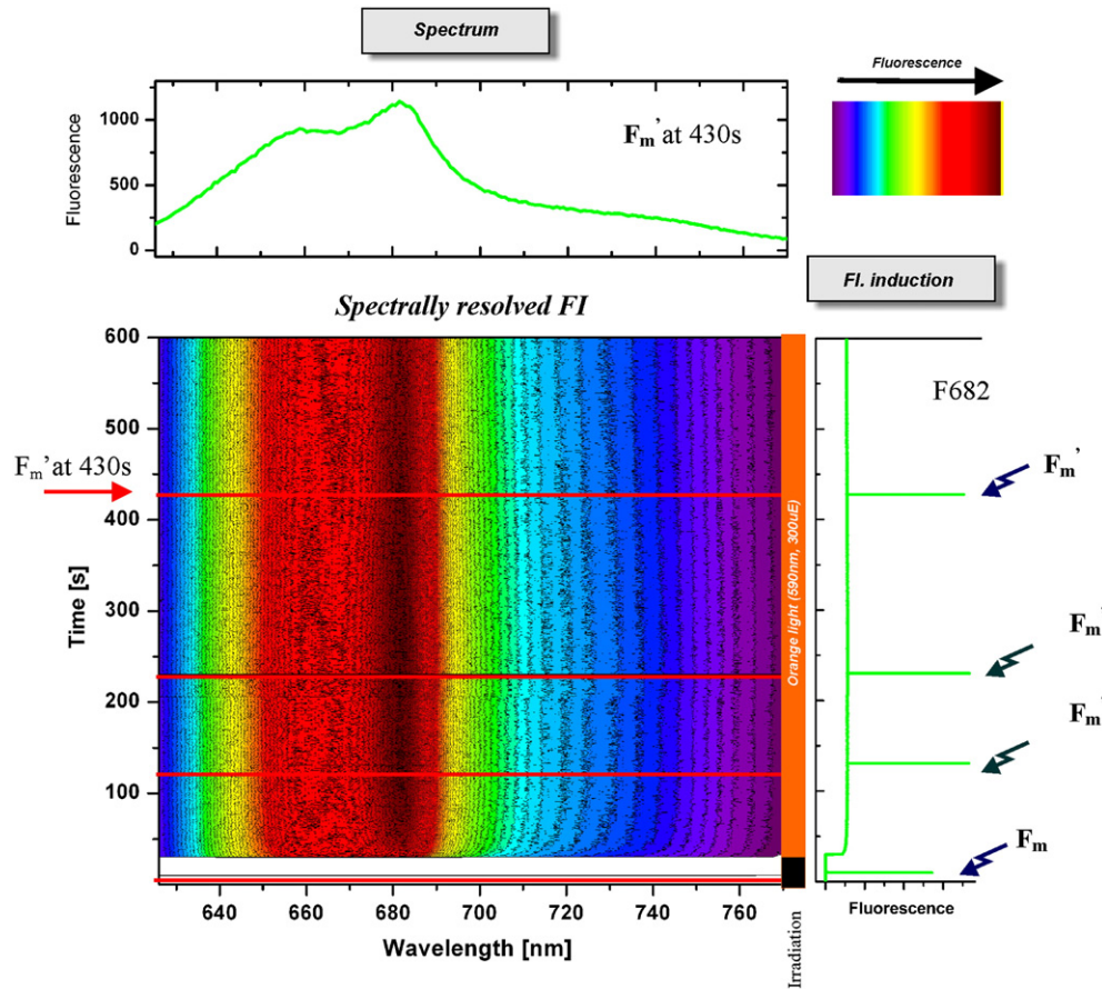
Fig. 4. A typical two dimensional (2D) plot of Spectrally Resolved Fluorescence Induction (SRFI) of WT Synechocystis sp. PCC 6803 in the presence of 10 \mu\text{M} DCMU. For this plot, raw fluorescence induction data were recorded with 20 min dark-adapted cells at room temperature. Fluorescence excitation, \lambda_e = 590 \text{ nm} , 300 \mu\text{mol photons m}^{-2} \text{ s}^{-1} , \Delta\lambda = 20 \text{ nm} . The graph shows F = f(\lambda, t) , where one dependent variable F (fluorescence intensity; color-coded isoemissive contours are plotted against two independent variables (wavelength ( \lambda ) in the range of 620 to 800 nm (the x-axis); and the time of illumination, t (s), in the range of 0–600 s; the y-axis). The entire spectrum was measured every 100 ms. Panel labeled as Spectrum (top, left) displays a section, parallel to the wavelength axis, at 200 s, whereas the panel Fl. Induction (right) displays fluorescence induction at selected wavelength (at 682 nm).
