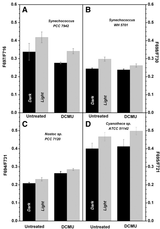
Fig. 9. The ratio of the 77 K fluorescence maxima of PS II/PS I measured with various phycobilisome-containing cyanobacteria. (A) Synechococcus PCC 7942 – here, fluorescence maximum of PSII was at 697 nm, and of PSI at 716 nm – thus, F697/F716 reflects fluorescence ratio of PS II/PS I; (B) Synechococcus WH 5701 – here, fluorescence maximum of PSII was at 698 nm, and that of PSI at 730 nm – thus, F698/F730 reflects fluorescence ratio of PS II/PS I; (C) Nostoc sp. PCC 7120 – here, fluorescence maximum of PSII was at 694 nm, and that of PSI at 731 nm – thus, F694/F731 reflects fluorescence ratio of PS II/PS I; (D) Cyanothece ATCC 51142 – here, fluorescence maximum of PSII was situated at 695 nm, and that of PSI at 721 nm) – thus, F695/F721 reflects fluorescence ratio of PS II/PS I. Standard deviation bars are for n=3 .
