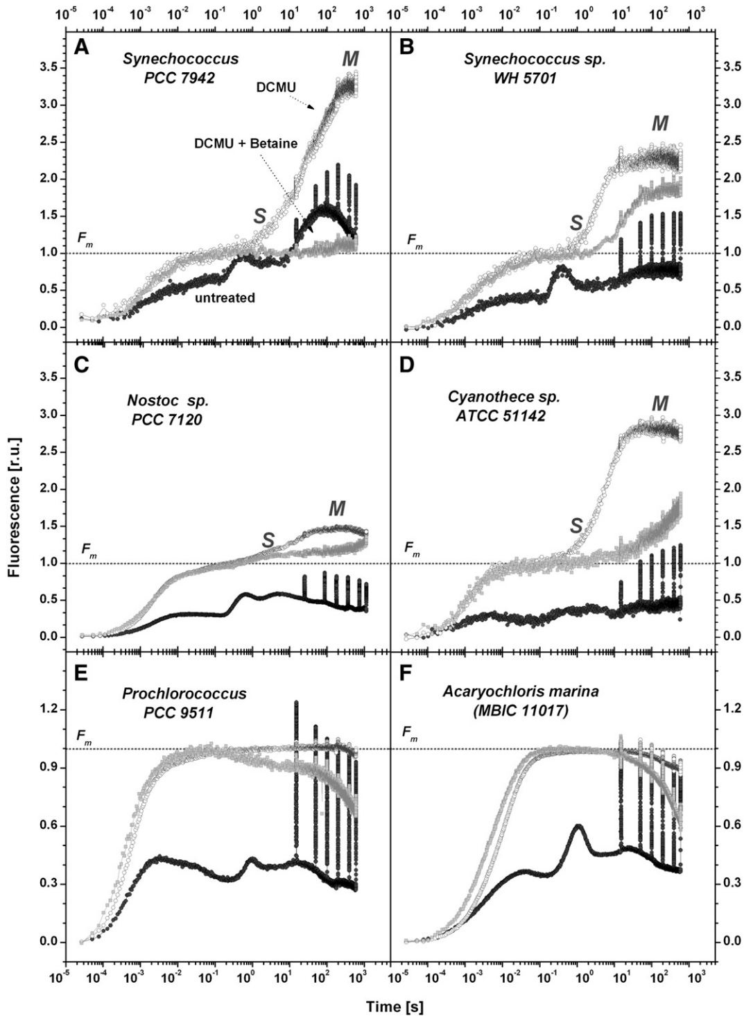
Fig. 8. Time course of chlorophyll a fluorescence changes measured with various cyanobacterial species as indicated. Samples without any addition ( untreated ; black line) or in the presence (as indicated) of DCMU (10 \mu M), nigericin (60 \mu M) and glycine betaine ( Betaine , 500 mM). Six saturation light pulses were applied at 15 s, 50 s, 200 s, 430 s and 600 s to obtain F_m . Data are normalized to the maximal fluorescence obtained after exciting samples with a saturating excitation pulse given before recording the fluorescence time course (see F_m line). The S and M levels during the slow fluorescence transient are marked; see panel A for the key to different treatments for all other panels.
