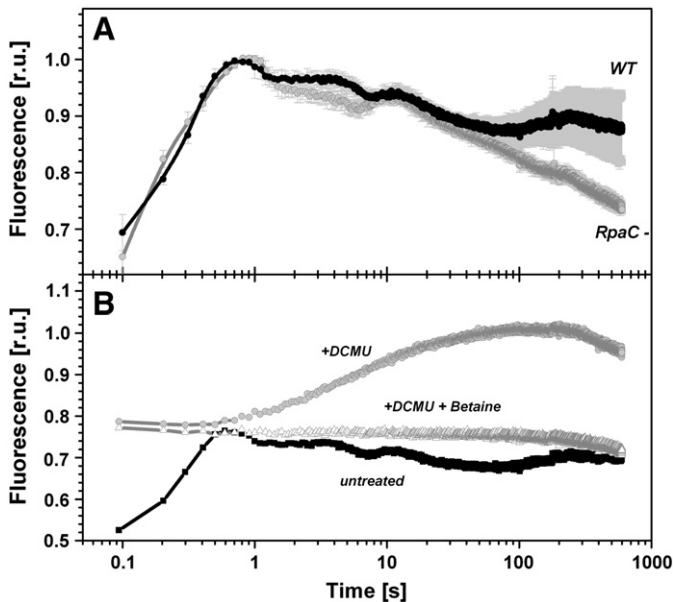
Fig. 6. Room temperature fluorescence induction measured at 682 nm (F682) with WT and RpaC - mutant of Synechocystis sp. PCC 6803. Panel A: comparison of WT and RpaC - induction of F682. Panel B: F682 induction of WT cells without any addition ( untreated ), with 10 \mu\text{M DCMU} ( DCMU ) and with 10 \mu\text{M DCMU} and 0.5 \text{ M glycine betaine} ( +DCMU + Betaine ). Data were obtained from spectrally resolved fluorescence induction (SRFI – for further details, see Fig. 4) method with orange actinic excitation ( 590 nm, \Delta\lambda = 20 nm, 300 \mu\text{mol photons m}^{-2} \text{s}^{-1} ). Data in the Panel A represent average of 3 independent measurements; SD of particular points are marked by gray color.
