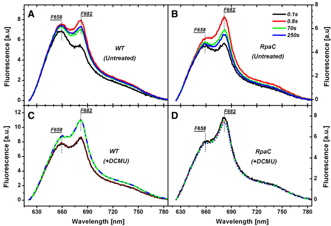
Fig. 5. Room temperature fluorescence spectra at specific times of the fluorescence induction curves of WT (A and C) and RpaC - mutant (B and D) of Synechocystis sp. PCC 6803. The spectra were measured by SRFI method at selected times (corresponding phases of the fluorescence induction, see Fig. 3): 0.1 s (I to P in -DCMU cells); 0.8 s (P level in \pm DCMU cells); 70 s (P to S in -DCMU cells, nearly M in +DCMU cells); 250 s (P to S in DCMU cells, M in +DCMU cells). Fluorescence excitation, \lambda_e = 590 nm, 300 \mu\text{mol photons m}^{-2} \text{s}^{-1} , \Delta\lambda = 20 nm. See Fig. 4 for further details.
