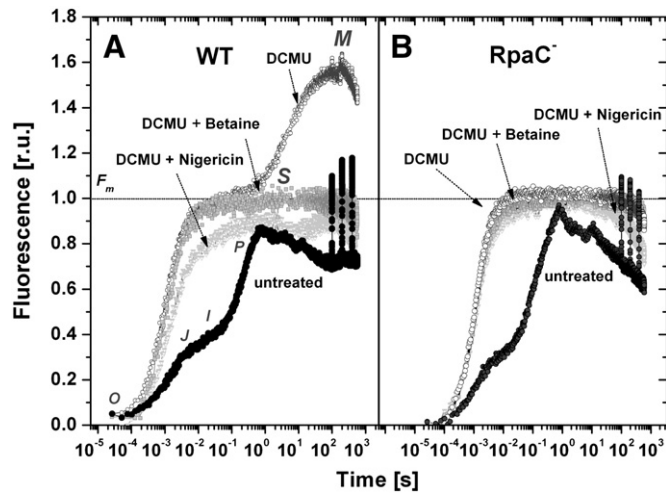
Fig. 3. Time course of chlorophyll a fluorescence measured with WT (A) or RpaC - mutant (B) of Synechocystis sp. PCC 6803. Samples without any addition ( untreated ) or in the presence (where indicated) of DCMU (10 \mu M), nigericin (60 \mu M) or glycine betaine (500 mM). Data are normalized to the maximal fluorescence obtained after the samples were excited with a saturating light pulse given just before the fluorescence time course was recorded. Three saturation pulses were applied at 200 s, 430 s and 600 s to obtain F_m (maximum fluorescence in light). Characteristic inflections and peaks (O–J–I–P–S–M) during the fluorescence transient are marked in two of the curves of panel A. Fluorescence excitation, \lambda_e = 590 nm, \Delta\lambda = \pm 20 nm (amber diode).
