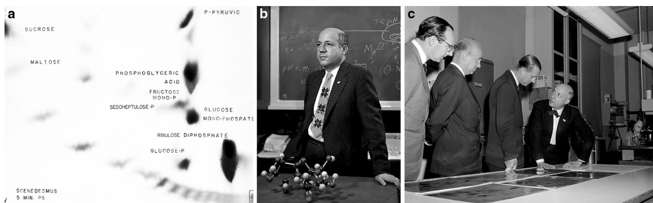
Fig. 8 a X-ray films exposed to 2-Dimensional paper chromatography resulted in autoradiograms. In this plate, key metabolites were labeled with ^{14}\text{CO}_2 within 5 min of photosynthesis, such as, ribulose biphosphate, clearly identified in the lower right corner. There would never have been a Calvin–Benson cycle without these autoradiograms developed by Benson. This plate was a teaching autoradiogram by Benson, circa 1960, now in the personal archive of AN. High resolution scientific photography by AN. b Melvin Calvin lecturing wearing a special tie with stylized ‘porphyrin rings’, his mother made for
